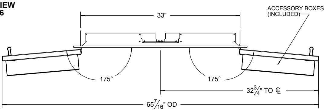
TOP VIEW AXE-42
