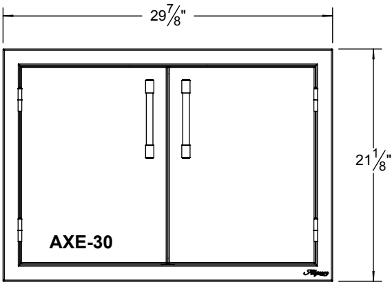
TOP VIEW AXE-30
