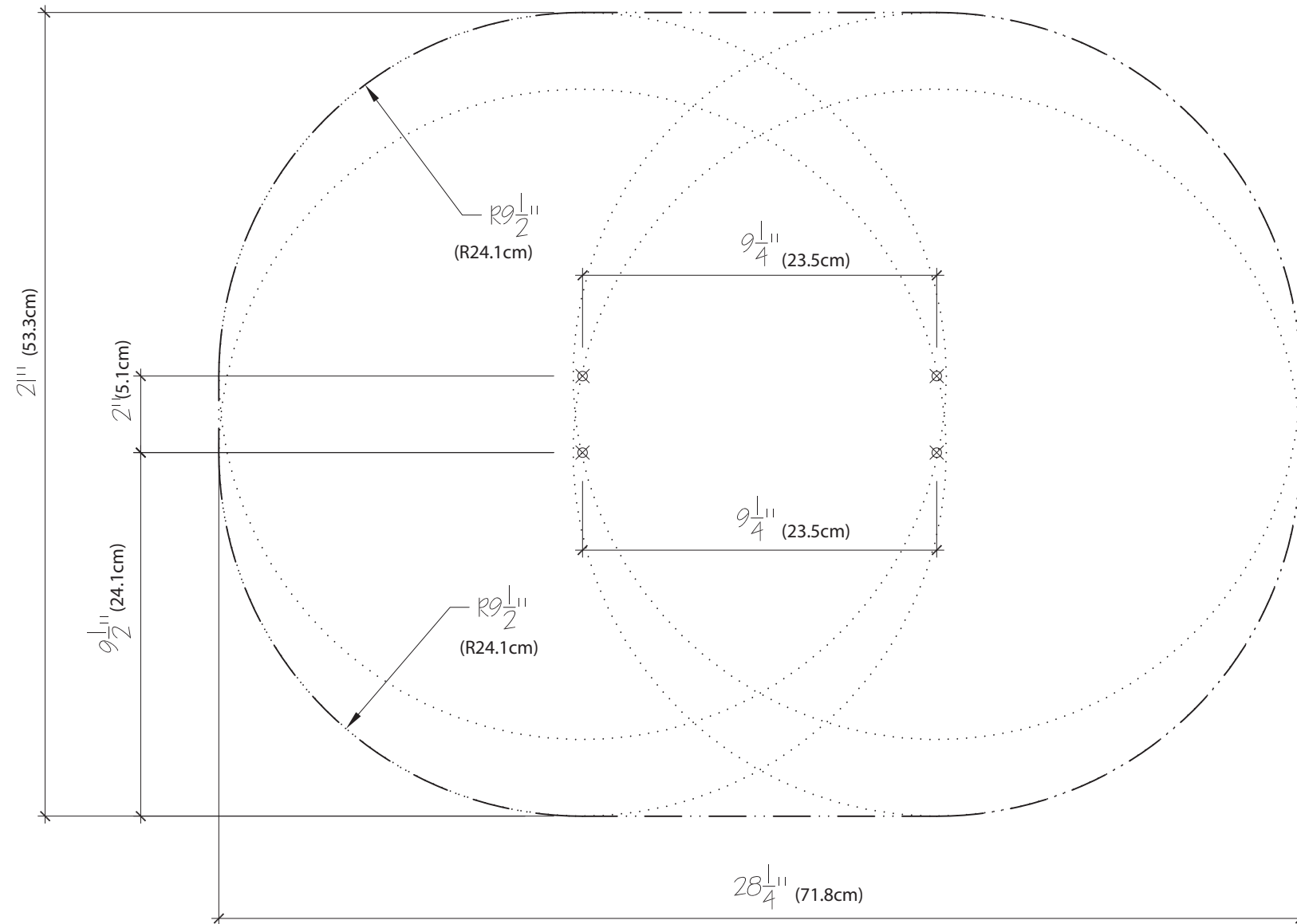
FIG. A - PLAN VIEW CUT-OUT
